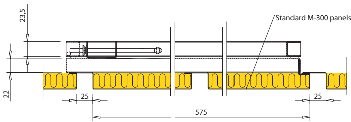
SECTION A-A, INSULATED FOR B-0 RATING.
