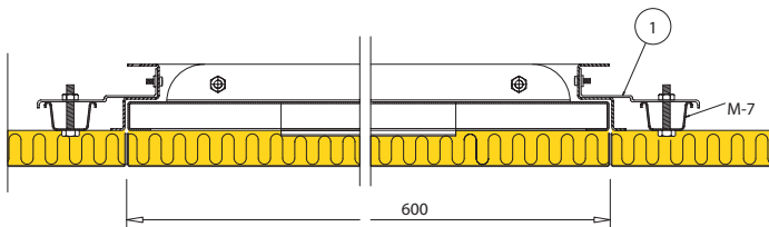
SECTION B-B, INSULATED FOR B-0 RATING.
